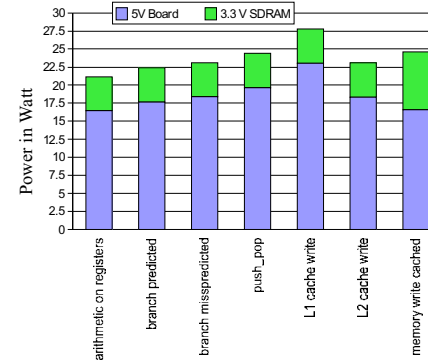
FIG. 1 : PC Board (PIII 866, 1 GB) Power Breakdown
