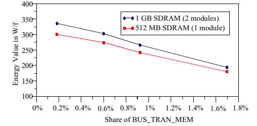
FIG. 8 : Energy values for SDRAM in relation to the transaction frequency.
