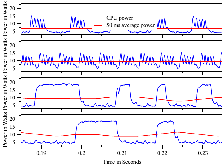
FIG. 12 :Throttled Apache to 10 Watt Limit (100, 200,300, 400 connection_attempts/s * 5 requests)
