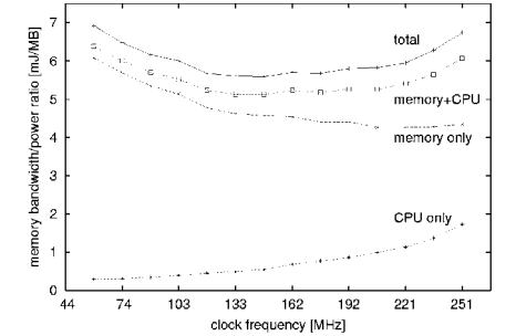
FIG. 2 : Energy breakdown for memory read (SA-1100 with 32 MB of EDO RAM) Measurements of the University of Delft [25]
