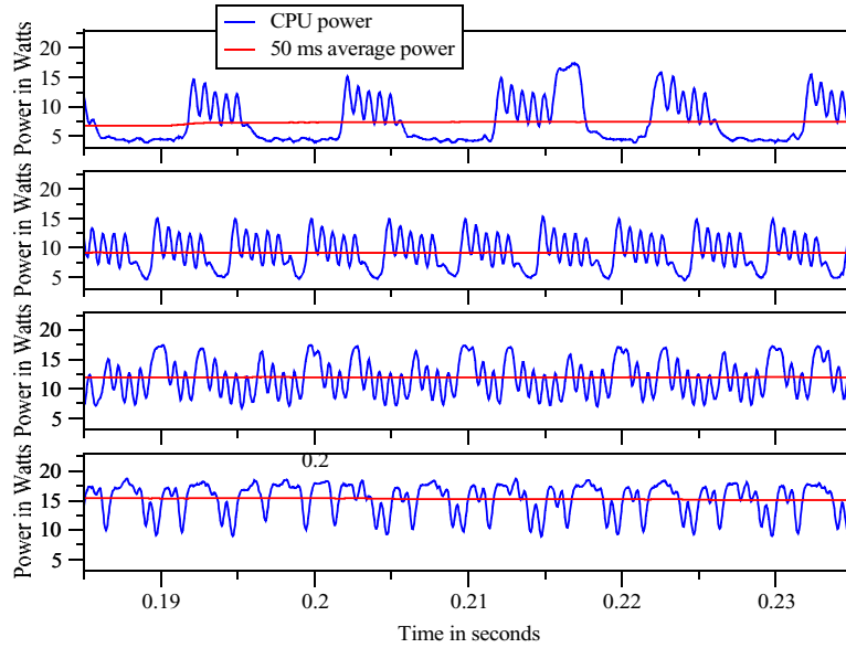
FIG. 11 :Unthrottled Apache (100-400 con/s * 5 requests)
