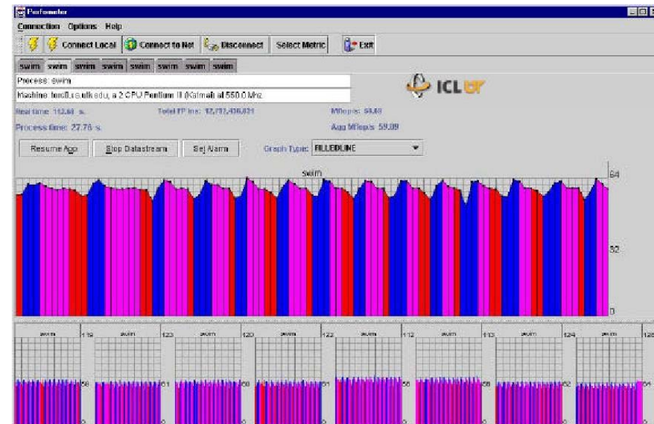
Figure 3. Perfometer monitoring a parallel application
