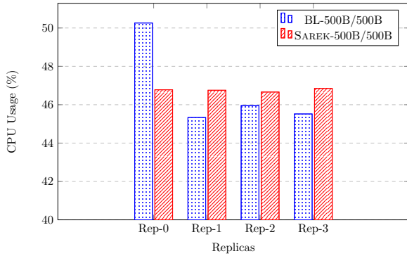
Fig. 11: CPU usage.
