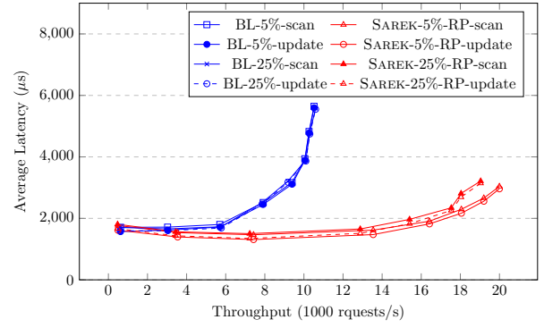
Fig. 13: Throughput and latency of scan/update workload.
