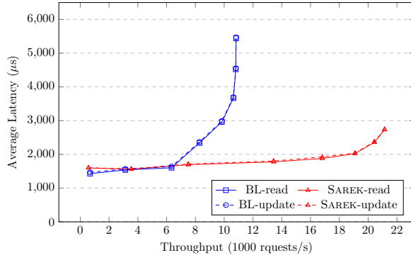
Fig. 12: Throughput and latency of read/update workload.
