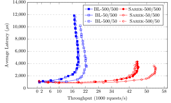
Fig. 6: Throughput and latency of simple requests.
