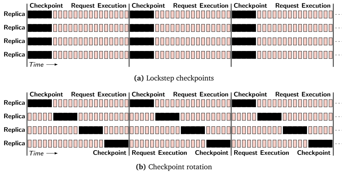
Figure 5.2: Comparison of state-of-the-art checkpointing techniques
