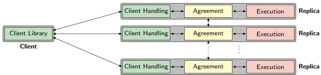
Figure 2.2: Overview of replication system software modules
