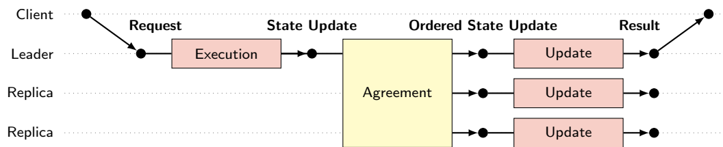
(b) Passive replication
