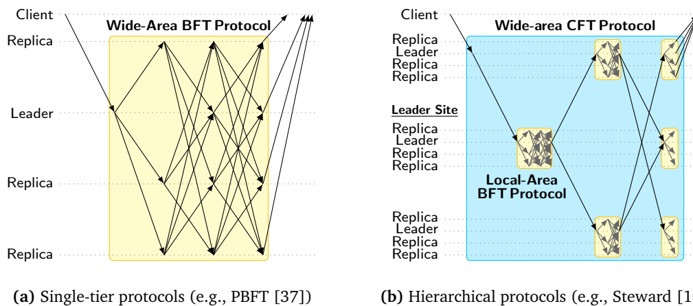
Figure 5.4: Message flow in wide-area environments for state-of-the-art replication protocols
