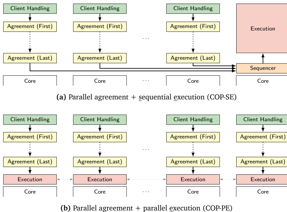
Figure 3.2: Replica architectures based on consensus-oriented parallelization
