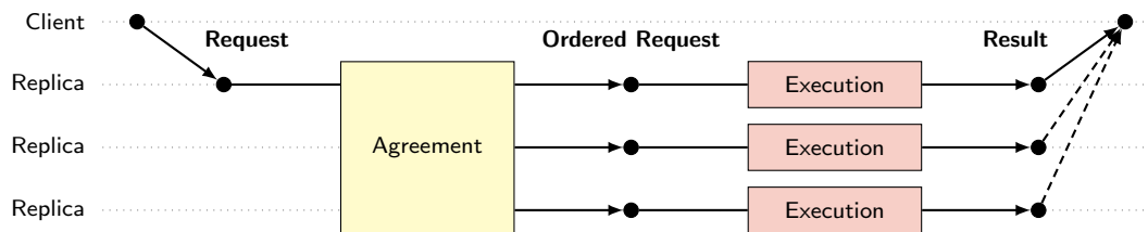
(a) Active replication
