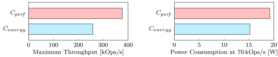
Figure 4.1: Measurement results for two configurations of a key-value store [63]
