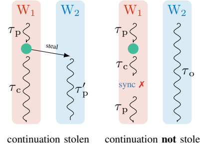
(c) Continuation-Stealing
