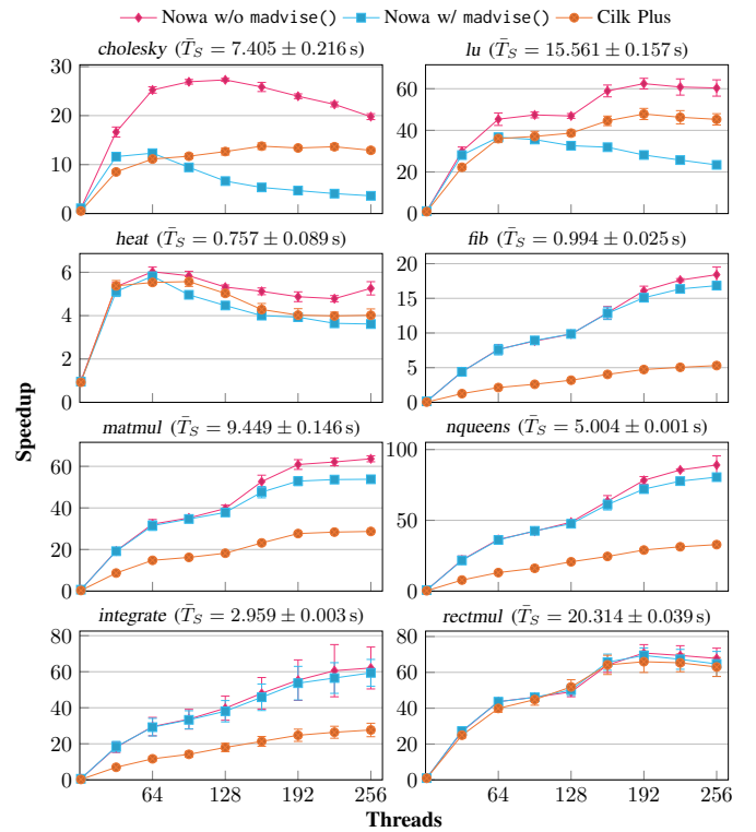
Figure 8: Comparison of the impact of madvise()
