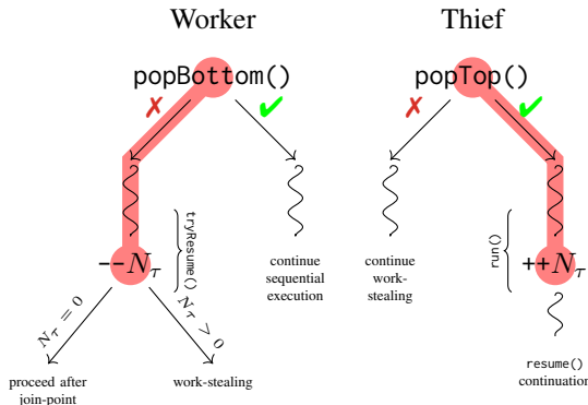
Figure 6: The data race between worker and thieves
