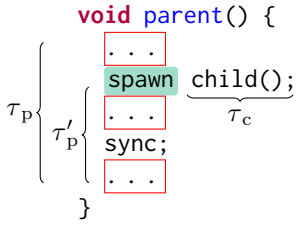
(a) Parent task \tau_P , Continuation (of parent task) \tau'_P , and Child \tau_c
