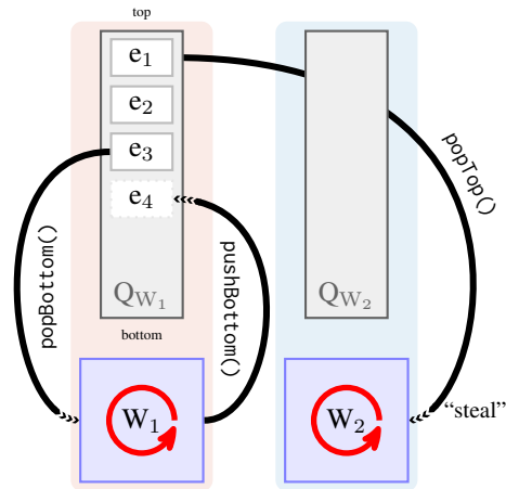
Figure 2: Workers and associated work-stealing queues
