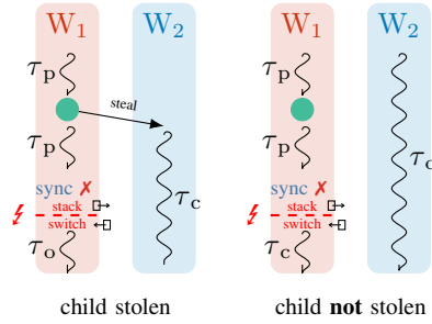
(b) Child-Stealing
