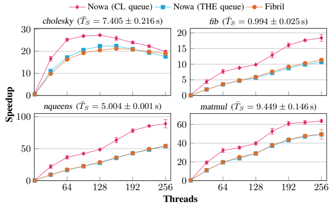
Figure 9: Comparison of the CL queue versus THE queue
