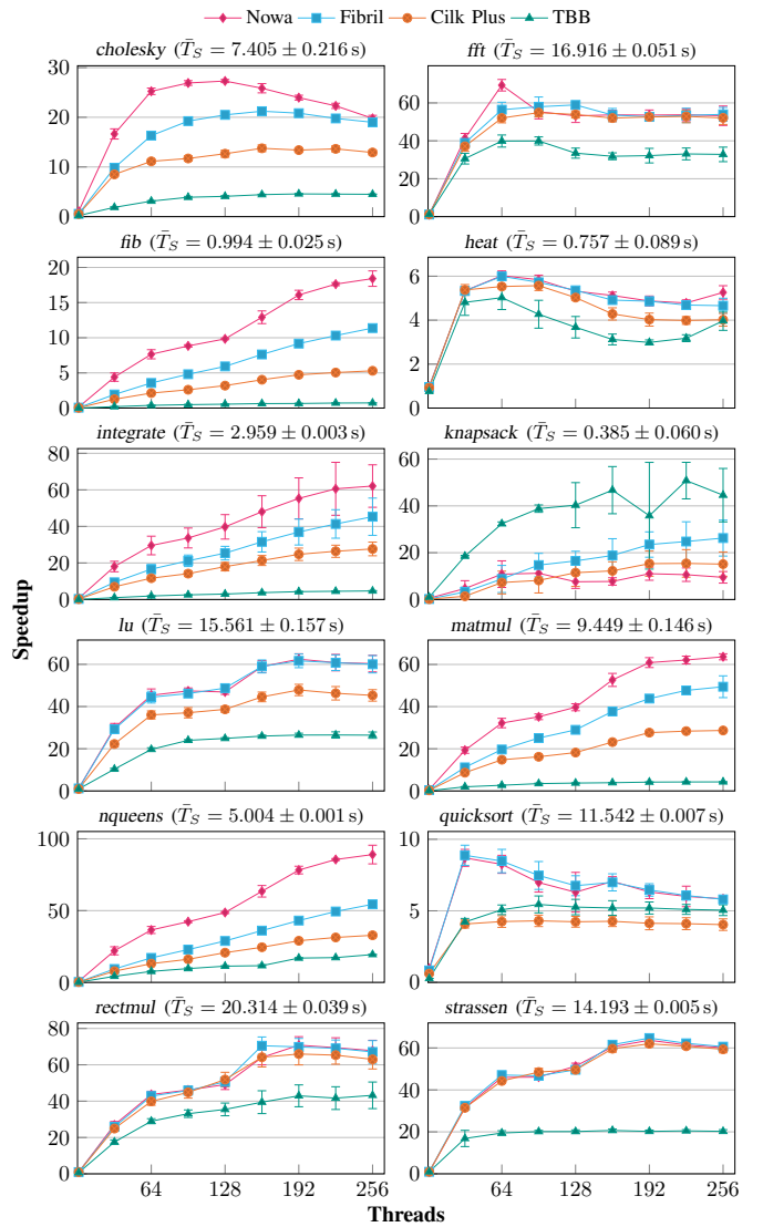
Figure 7: Speedup using 1–256 hardware threads
