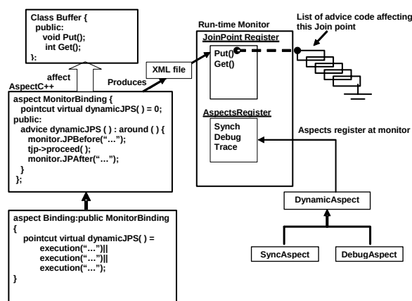
Figure 4 AspectC++ dynamic weaving framework
